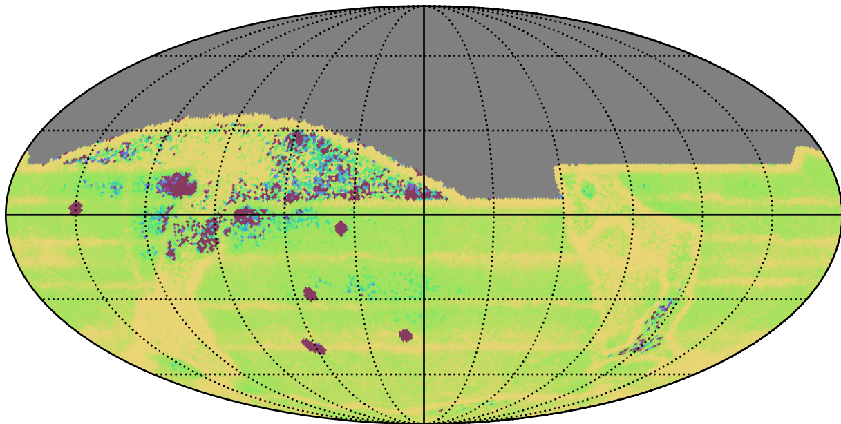
early_ss_template_fpextra3.0_v3.4_10yrs All sky: Median Intra-Night Gap
