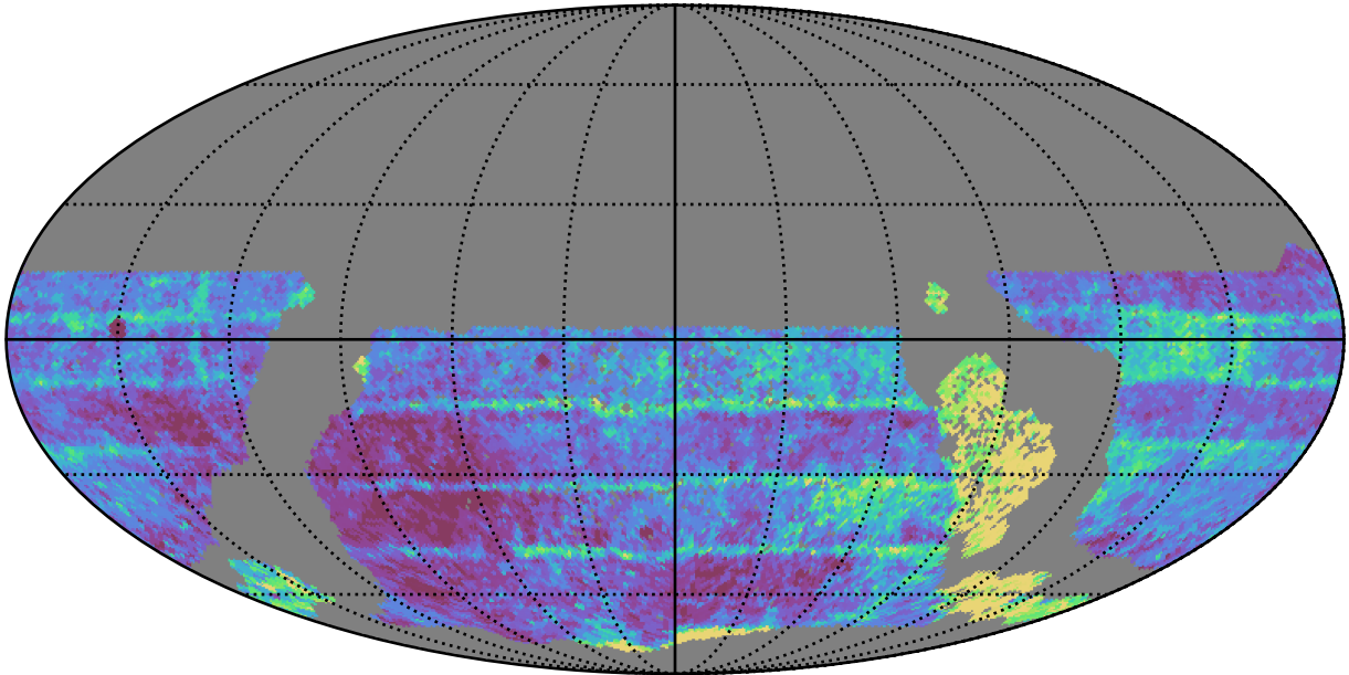
early_ss_template_fpextra3.0_v3.4_10yrs WFD z band: Median Inter-Night Gap
