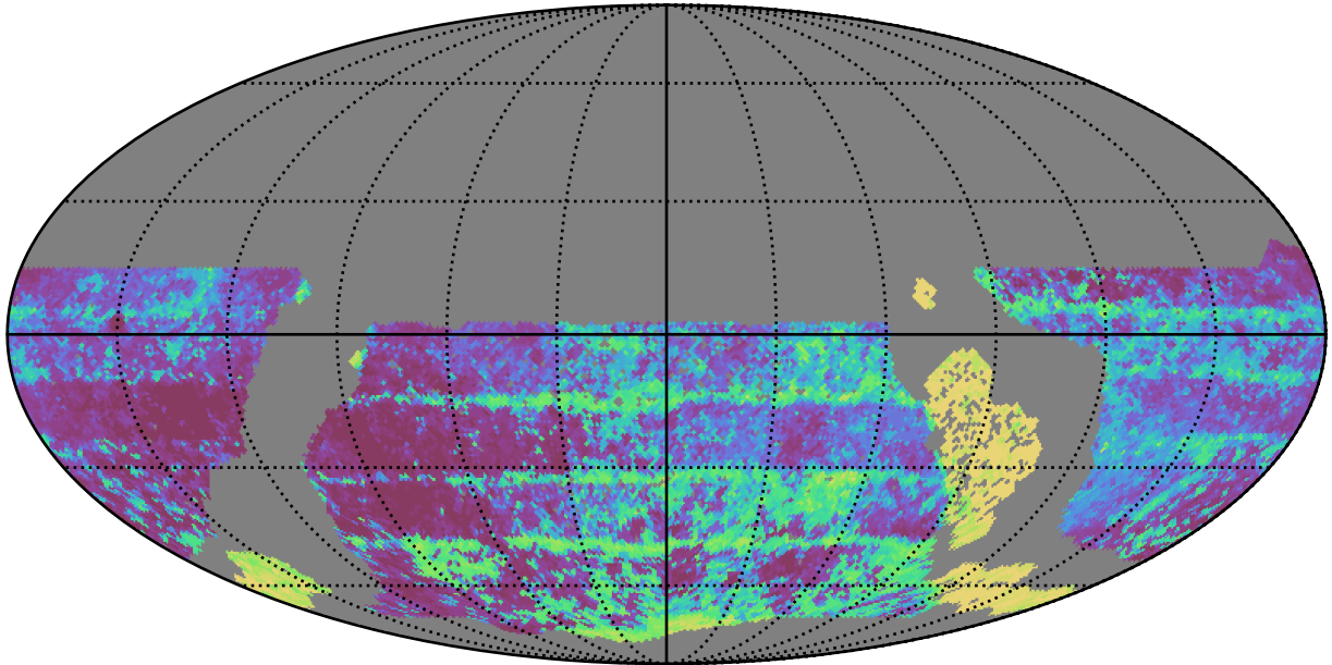
early_ss_template_fpextra3.0_v3.4_10yrs WFD y band: Median Inter-Night Gap
