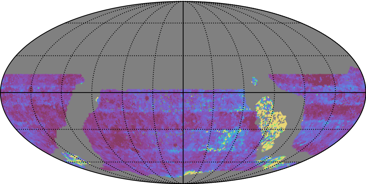
early_ss_template_fpextra3.0_v3.4_10yrs WFD u band: Median Inter-Night Gap
