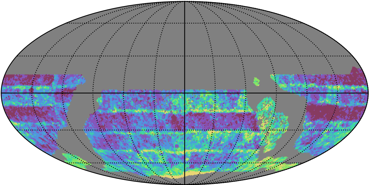
early_ss_template_fpextra3.0_v3.4_10yrs WFD r band: Median Inter-Night Gap
