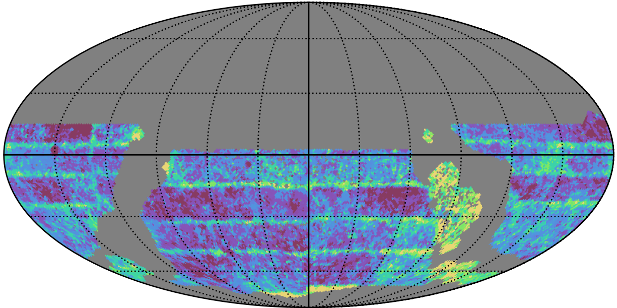
early_ss_template_fpextra3.0_v3.4_10yrs WFD i band: Median Inter-Night Gap
