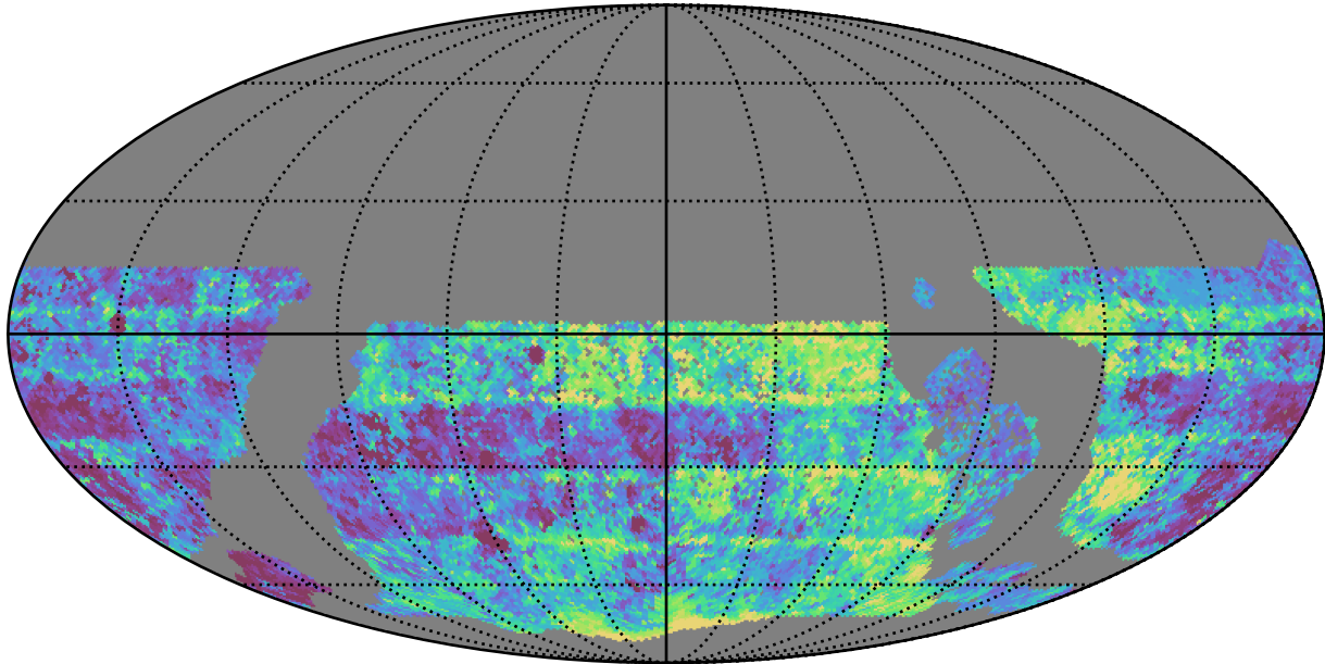
early_ss_template_fpextra3.0_v3.4_10yrs WFD g band: Median Inter-Night Gap
