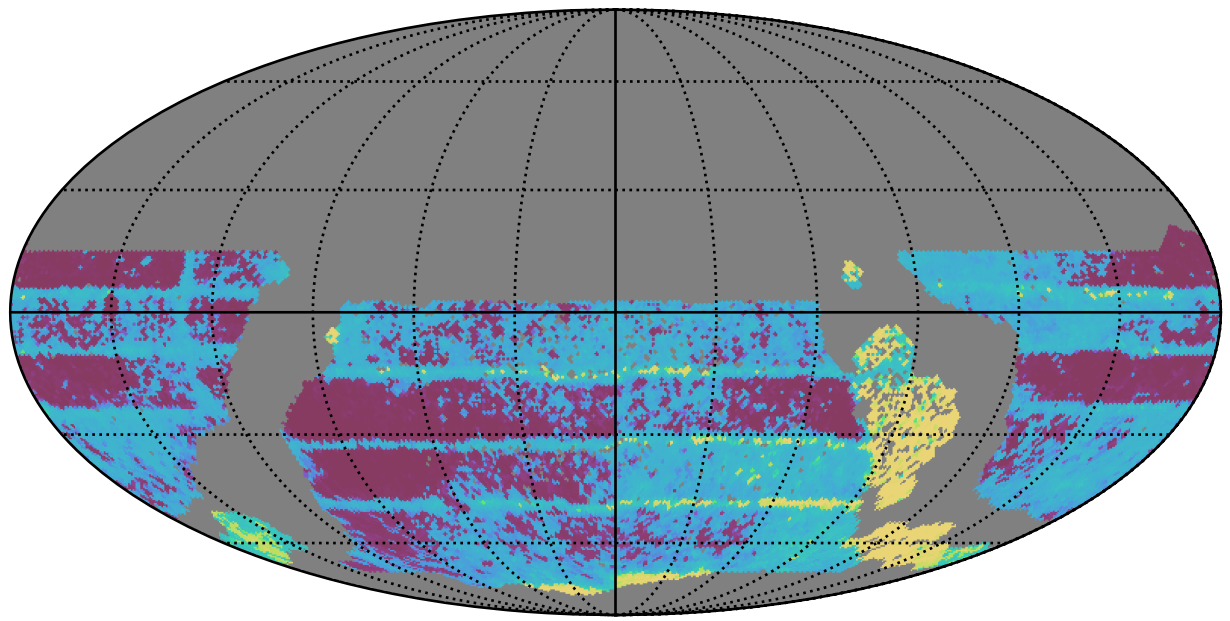
early_ss_template_fpextra3.0_v3.4_10yrs WFD all bands: Median Inter-Night Gap
