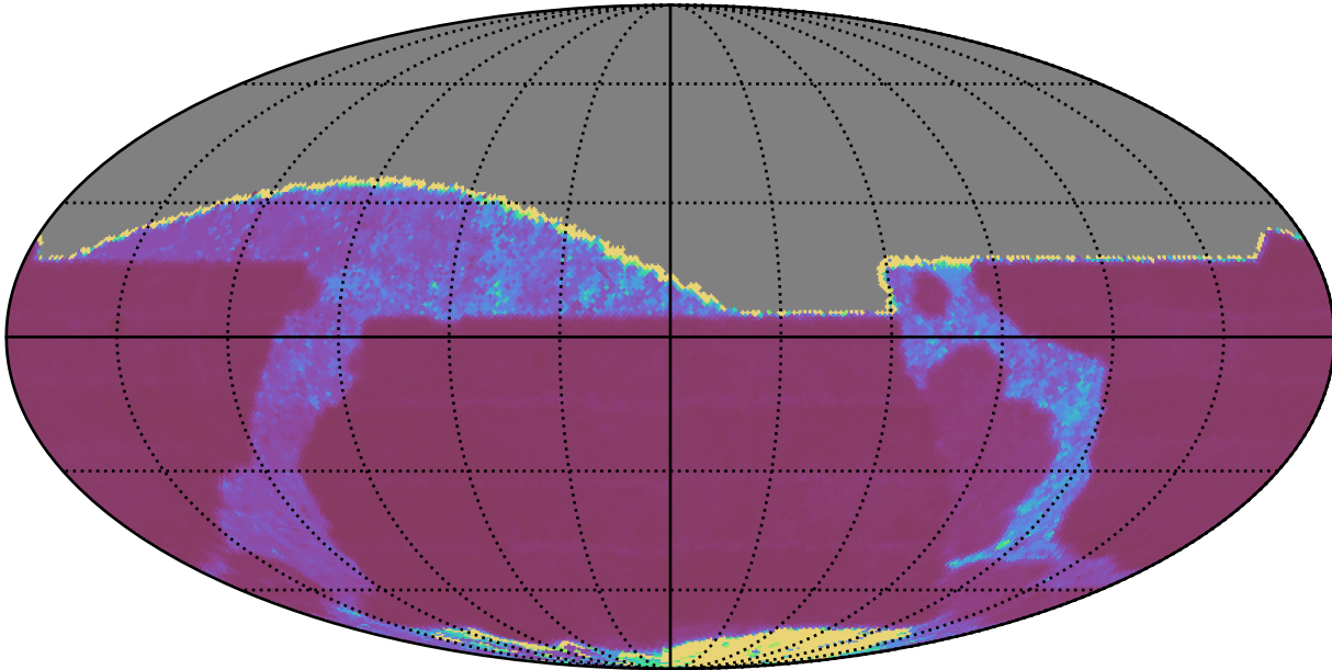
early_ss_template_fpextra3.0_v3.4_10yrs All sky z band: Median Inter-Night Gap
