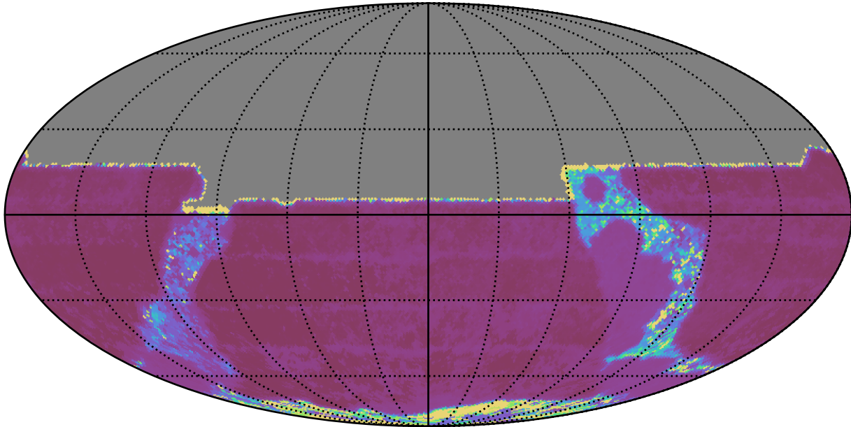
early_ss_template_fpextra3.0_v3.4_10yrs All sky y band: Median Inter-Night Gap
