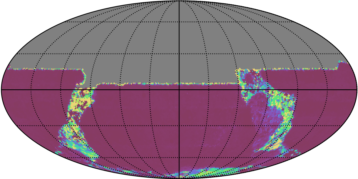
early_ss_template_fpextra3.0_v3.4_10yrs All sky u band: Median Inter-Night Gap
