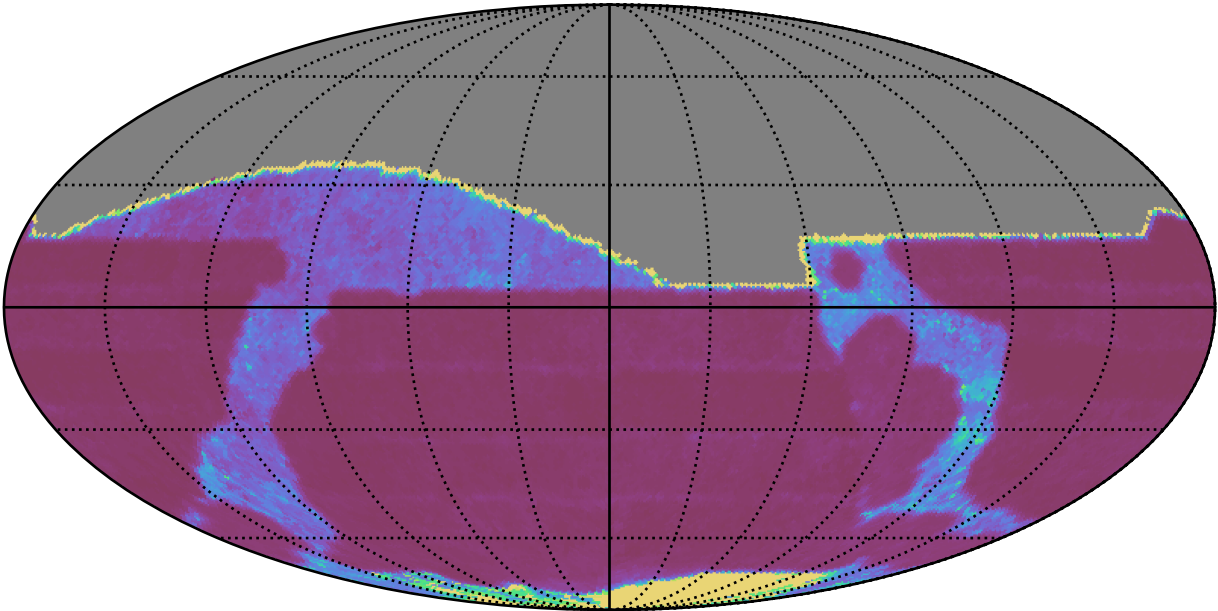
early_ss_template_fpextra3.0_v3.4_10yrs All sky r band: Median Inter-Night Gap
