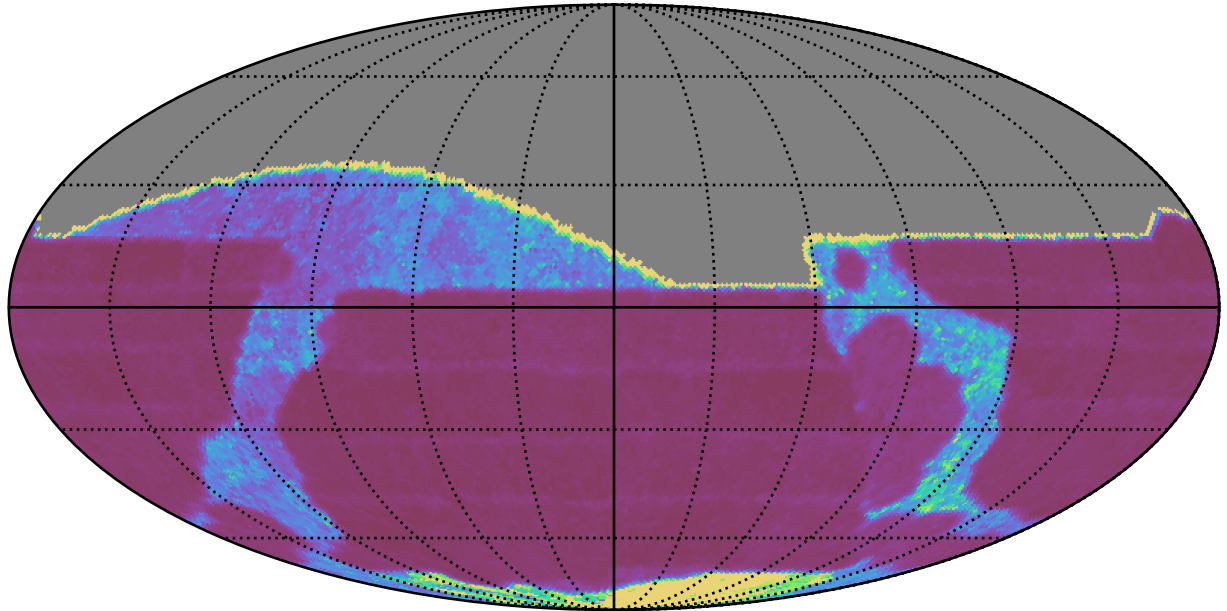
early_ss_template_fpextra3.0_v3.4_10yrs All sky i band: Median Inter-Night Gap
