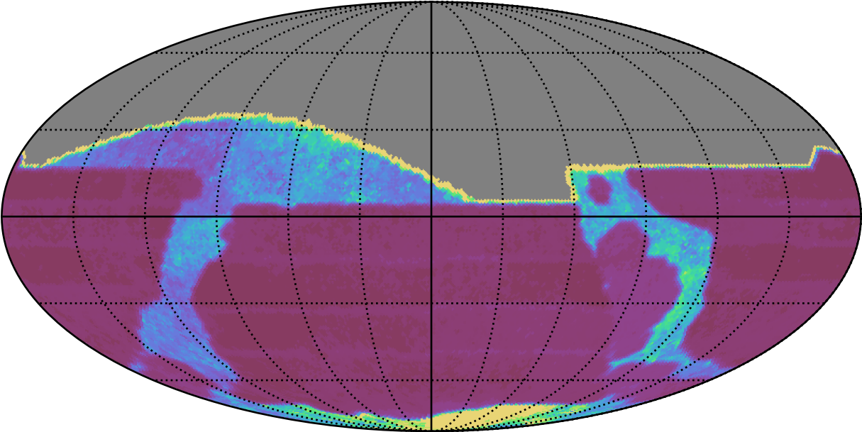
early_ss_template_fpextra3.0_v3.4_10yrs All sky all bands: Median Inter-Night Gap
