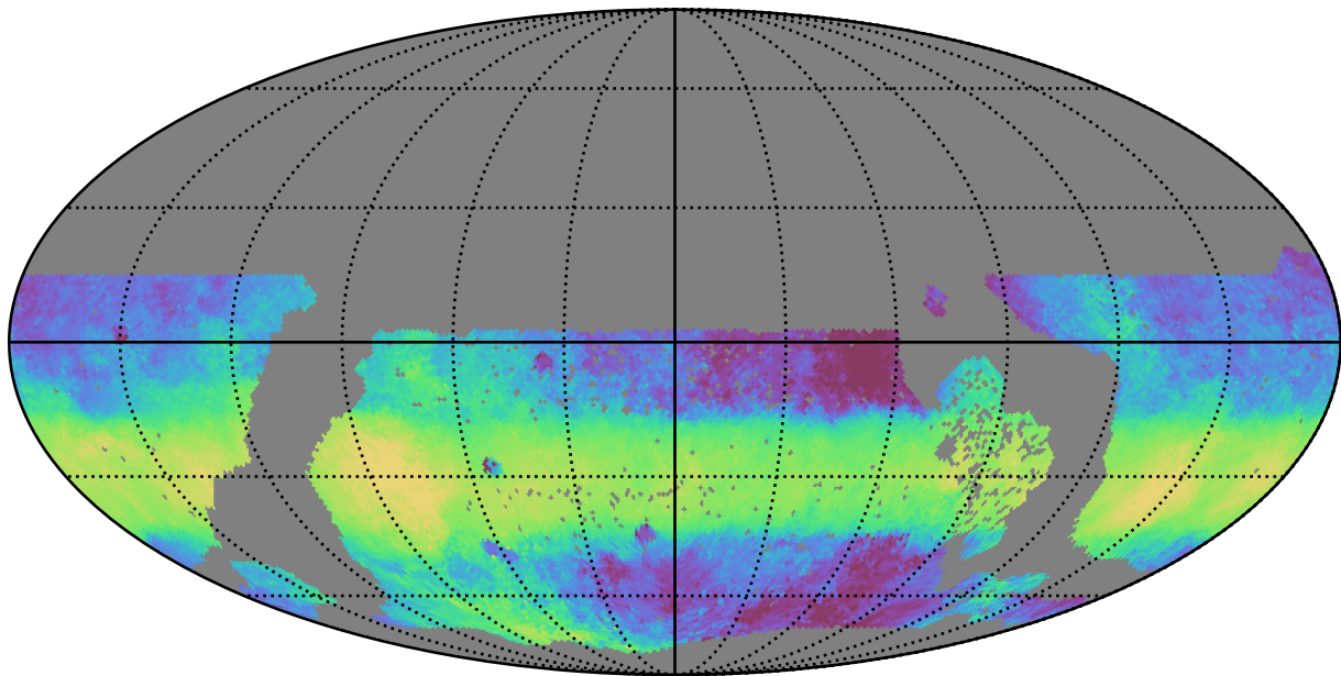
early_ss_template_fpextra3.0_v3.4_10yrs WFD y band: Median HA
