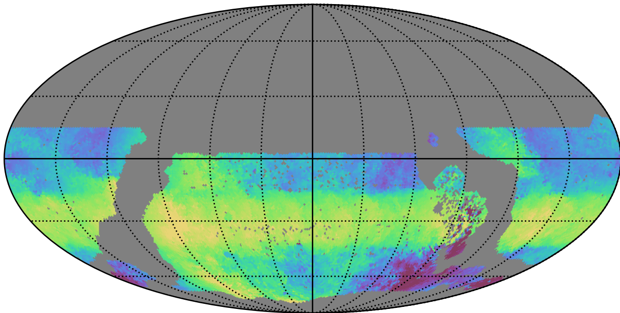
early_ss_template_fpextra3.0_v3.4_10yrs WFD u band: Median HA
