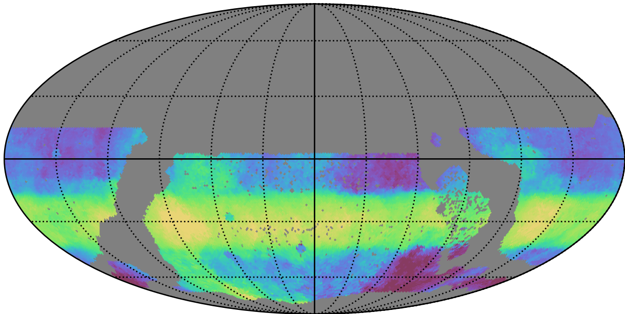
early_ss_template_fpextra3.0_v3.4_10yrs WFD r band: Median HA
