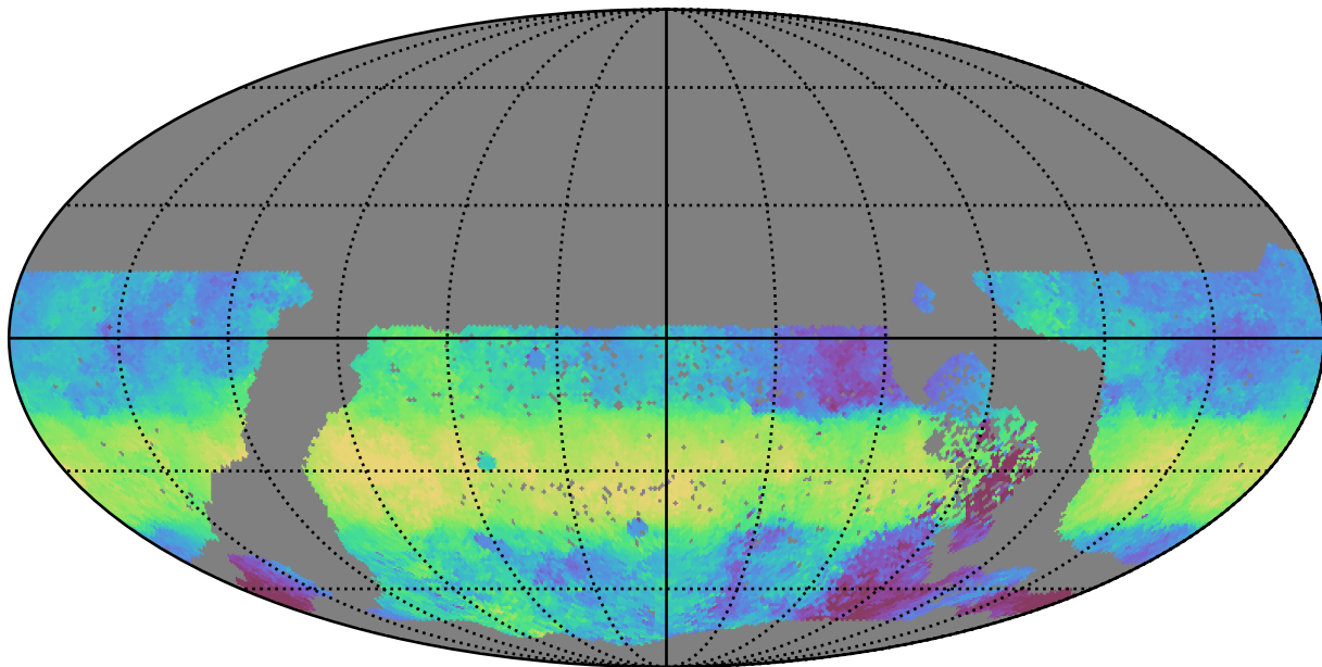
early_ss_template_fpextra3.0_v3.4_10yrs WFD g band: Median HA
