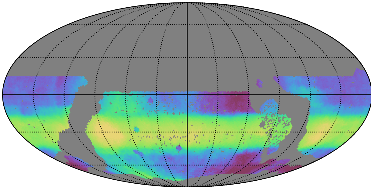
early_ss_template_fpextra3.0_v3.4_10yrs WFD all bands: Median HA
