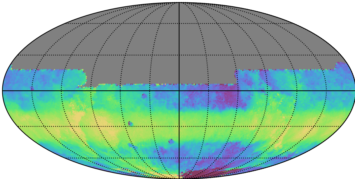
early_ss_template_fpextra3.0_v3.4_10yrs All sky y band: Median HA
