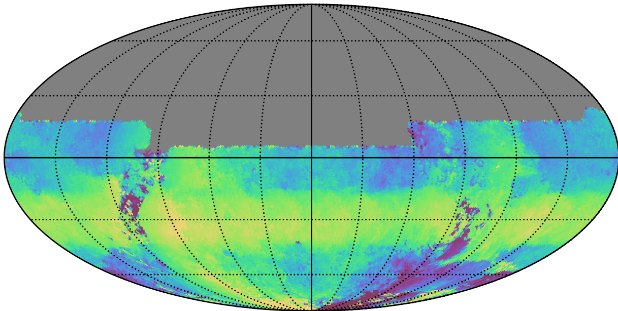
early_ss_template_fpextra3.0_v3.4_10yrs All sky u band: Median HA
