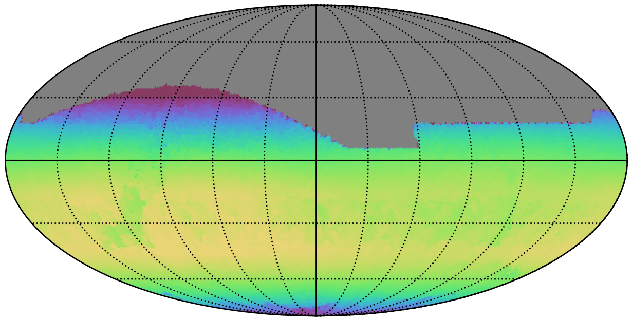
early_ss_template_fpextra3.0_v3.4_10yrs All sky z band: Max skyBrightness
