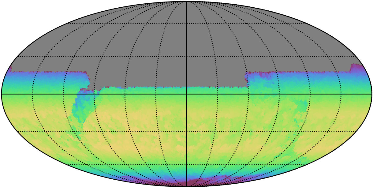
early_ss_template_fpextra3.0_v3.4_10yrs All sky y band: Max skyBrightness
