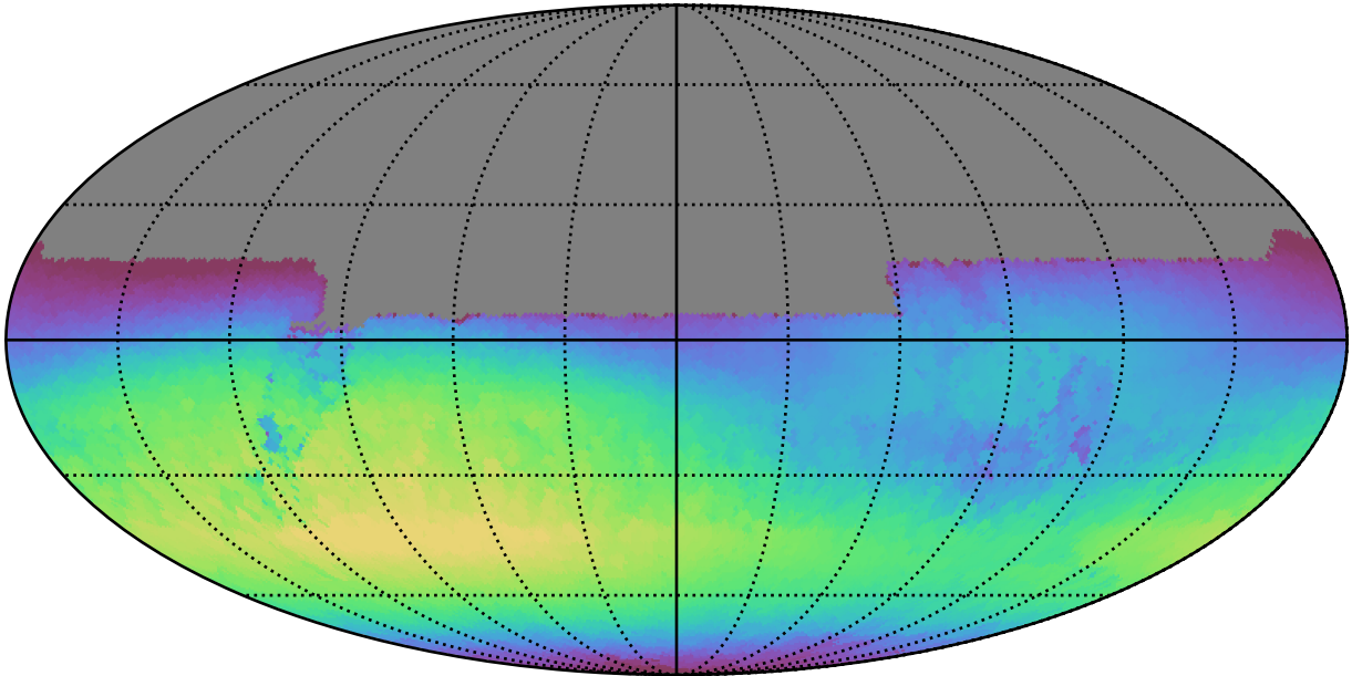
early_ss_template_fpextra3.0_v3.4_10yrs All sky u band: Max skyBrightness
