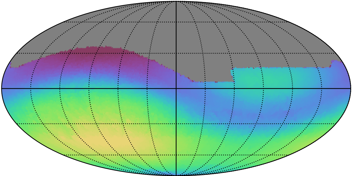
early_ss_template_fpextra3.0_v3.4_10yrs All sky g band: Max skyBrightness
