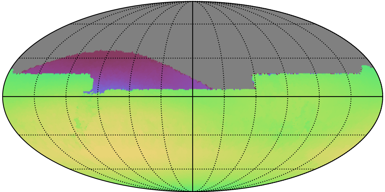
early_ss_template_fpextra3.0_v3.4_10yrs All sky all bands: Max skyBrightness
