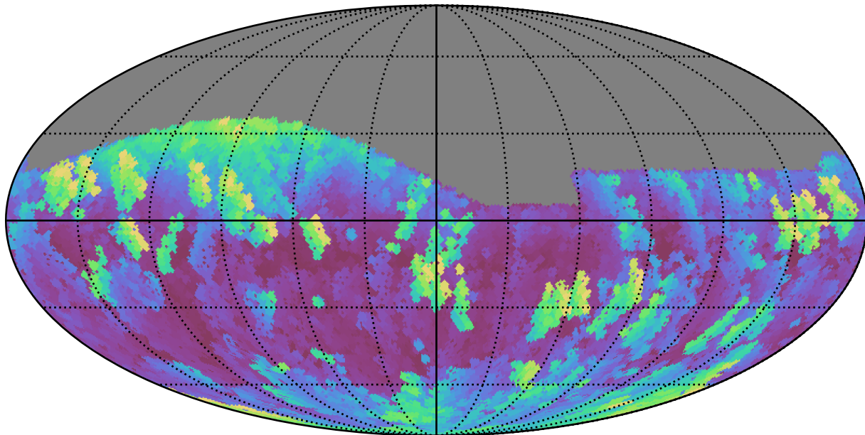
early_ss_template_fpextra3.0_v3.4_10yrs Yr 1 i band: Max airmass
