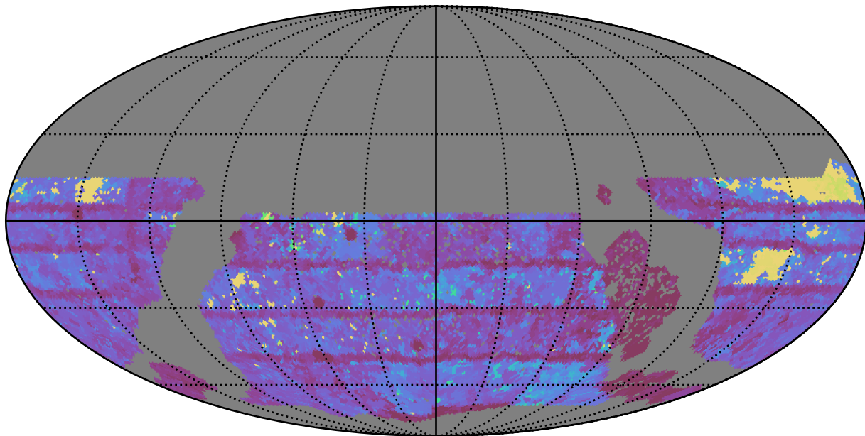
early_ss_template_fpextra3.0_v3.4_10yrs WFD r band: Max Inter-Night Gap
