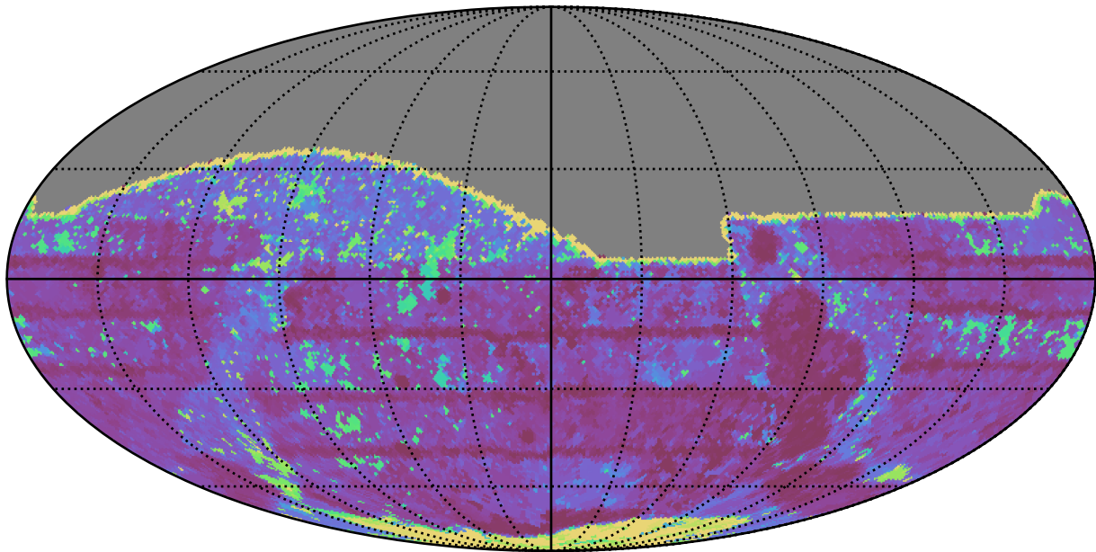
early_ss_template_fpextra3.0_v3.4_10yrs All sky z band: Max Inter-Night Gap
