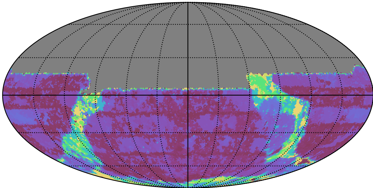
early_ss_template_fpextra3.0_v3.4_10yrs All sky u band: Max Inter-Night Gap
