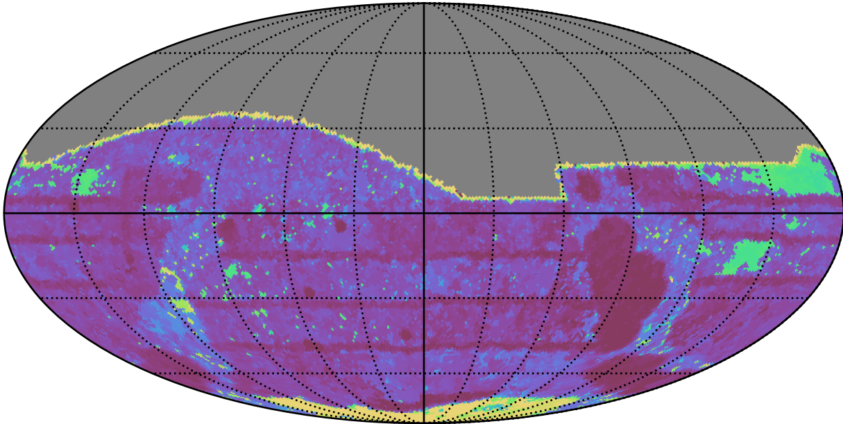
early_ss_template_fpextra3.0_v3.4_10yrs All sky r band: Max Inter-Night Gap
