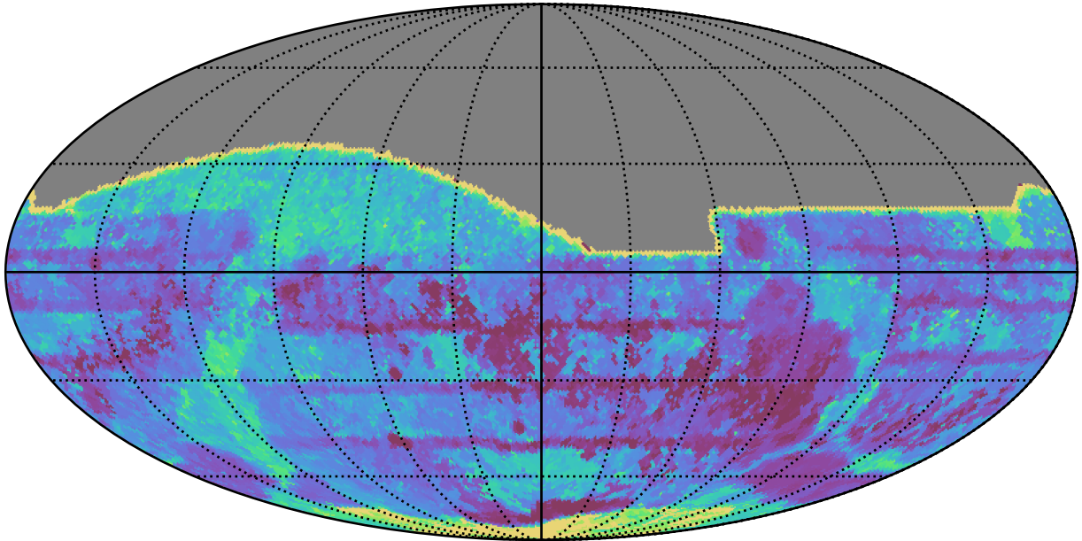
early_ss_template_fpextra3.0_v3.4_10yrs All sky all bands: Max Inter-Night Gap
