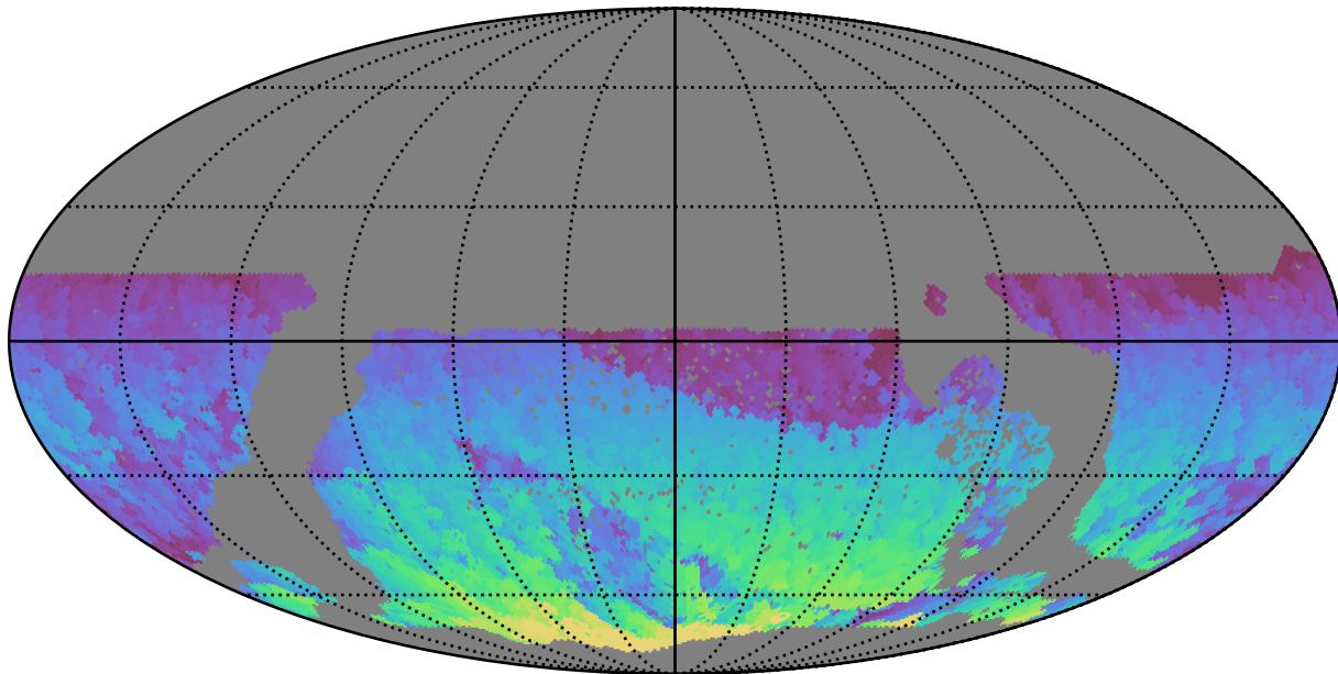
early_ss_template_fpextra3.0_v3.4_10yrs WFD z band: Max HA
