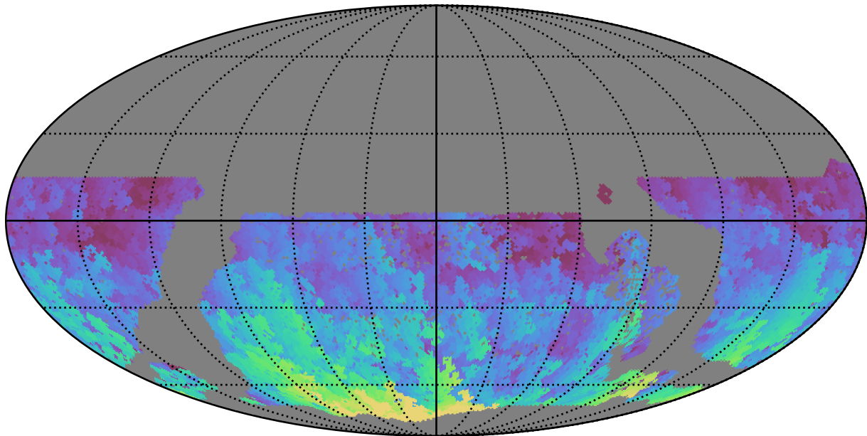
early_ss_template_fpextra3.0_v3.4_10yrs WFD u band: Max HA
