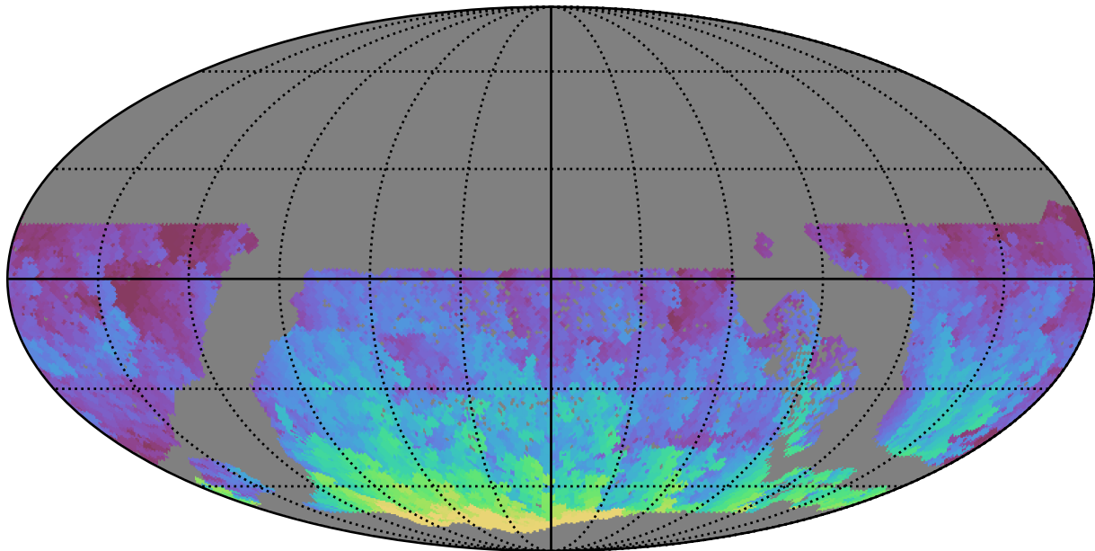
early_ss_template_fpextra3.0_v3.4_10yrs WFD r band: Max HA
