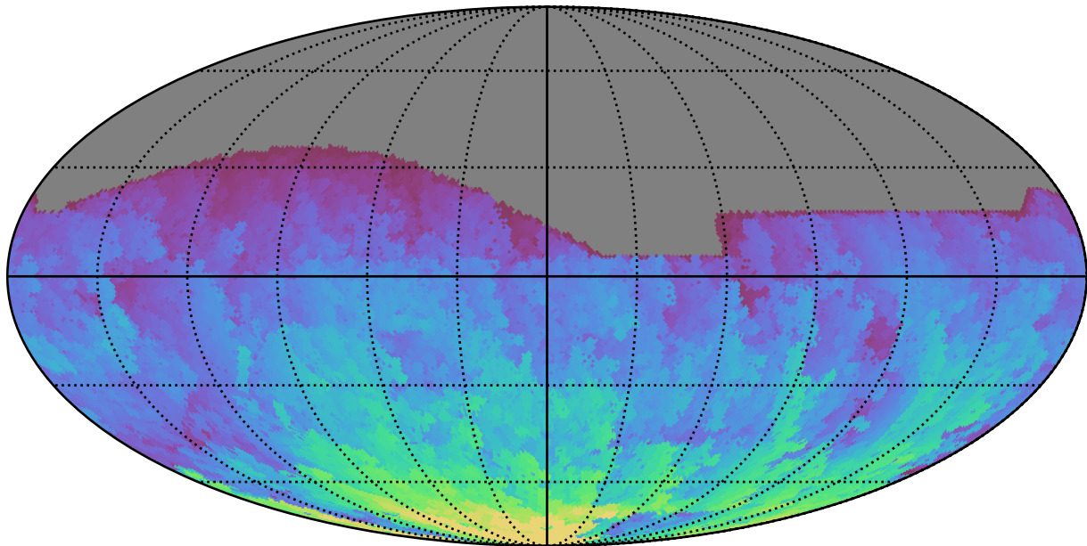
early_ss_template_fpextra3.0_v3.4_10yrs All sky r band: Max HA
