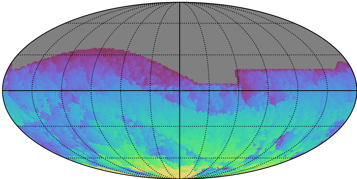
early_ss_template_fpextra3.0_v3.4_10yrs All sky i band: Max HA
