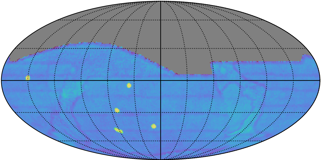
early_ss_template_fpextra3.0_v3.4_10yrs gri All sky: Fraction of visits with a revisit < 60 min
