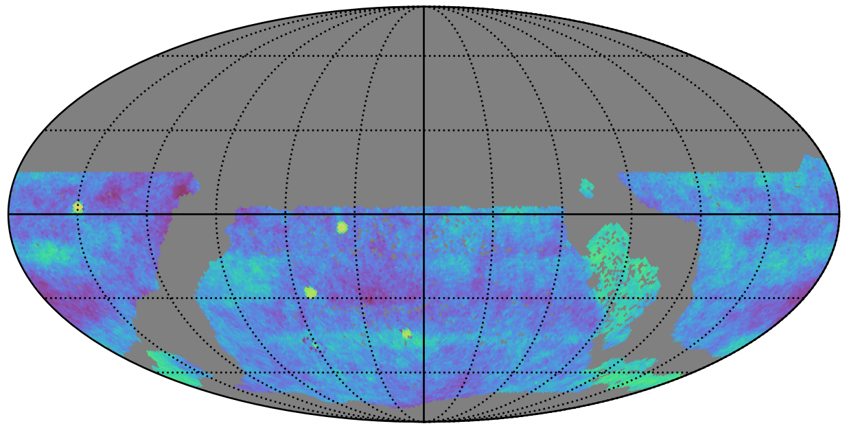
early_ss_template_fpextra3.0_v3.4_10yrs gri WFD: Fraction of visits in pairs (20-90 min)
