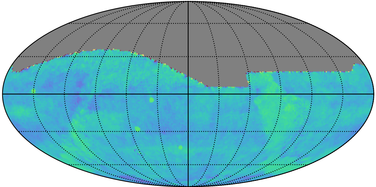
early_ss_template_fpextra3.0_v3.4_10yrs gri All sky: Fraction of visits in pairs (20-90 min)
