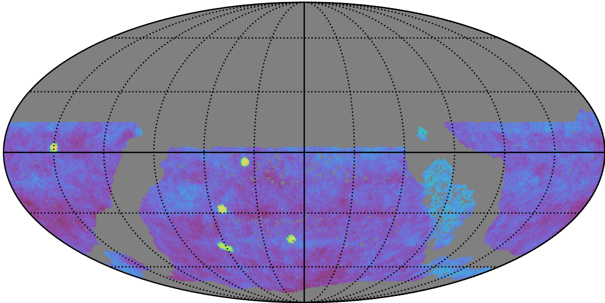
early_ss_template_fpextra3.0_v3.4_10yrs gri WFD: Fraction of visits in pairs (10-60 min)
