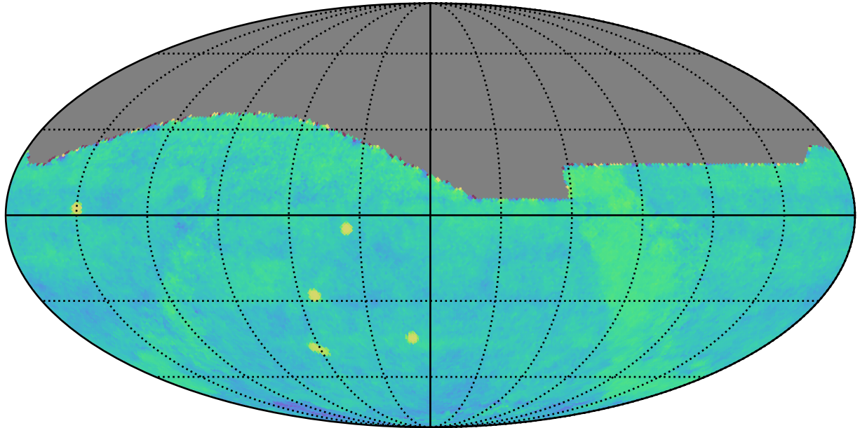
early_ss_template_fpextra3.0_v3.4_10yrs gri All sky: Fraction of visits in pairs (10-60 min)
