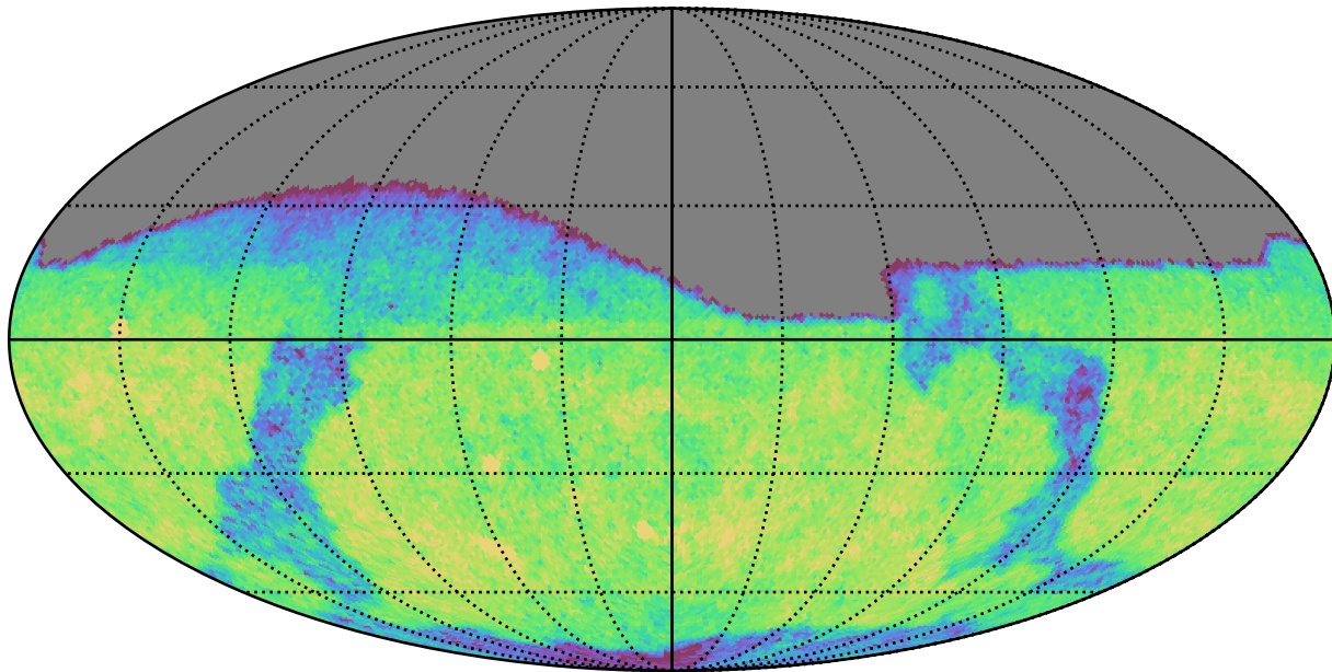
early_ss_template_fpextra3.0_v3.4_10yrs Yr 1 z band: CoaddM5
