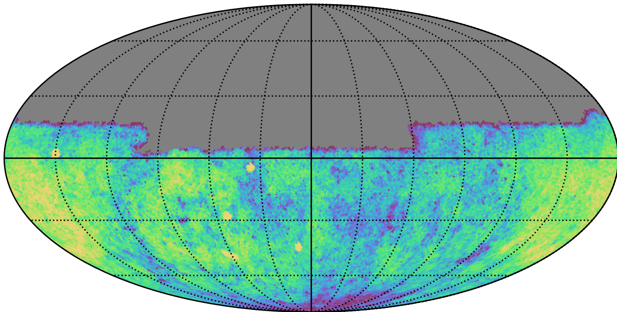
early_ss_template_fpextra3.0_v3.4_10yrs Yr 1 u band: CoaddM5
