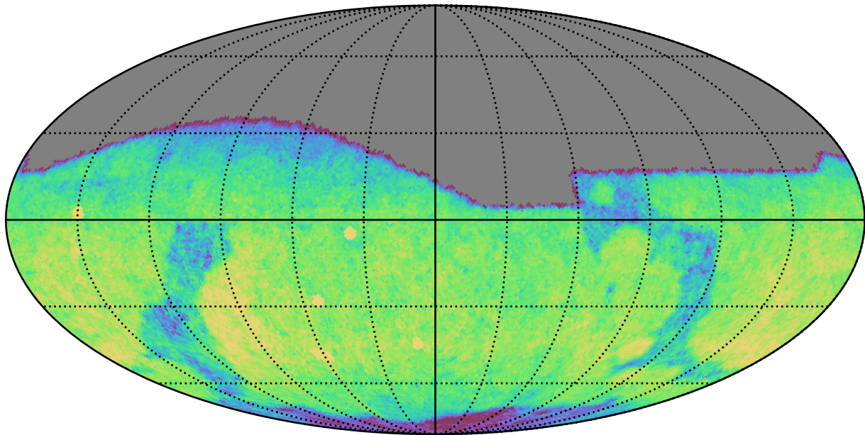
early_ss_template_fpextra3.0_v3.4_10yrs Yr 1 r band: CoaddM5
