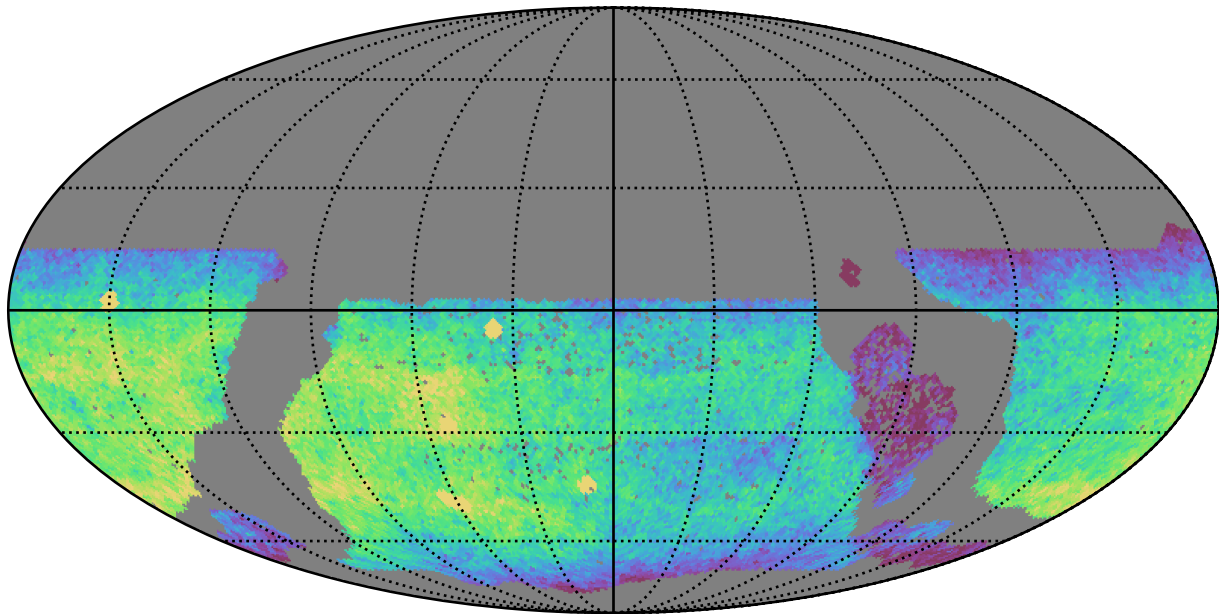
early_ss_template_fpextra3.0_v3.4_10yrs WFD u band: CoaddM5
