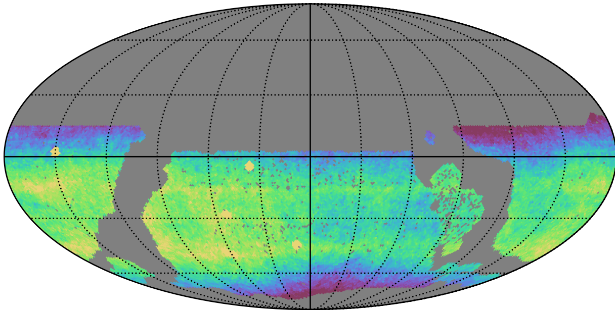
early_ss_template_fpextra3.0_v3.4_10yrs WFD i band: CoaddM5
