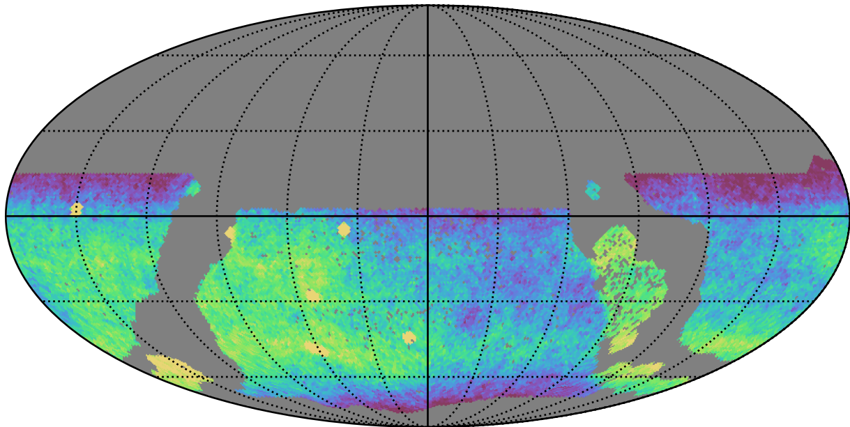
early_ss_template_fpextra3.0_v3.4_10yrs WFD g band: CoaddM5
