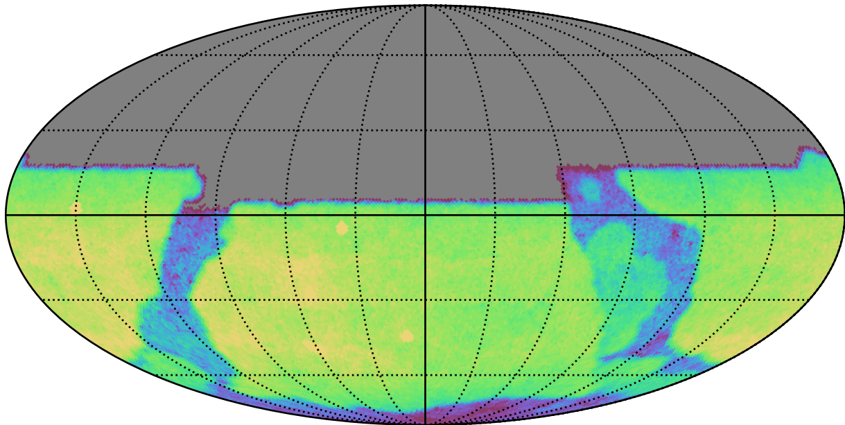
early_ss_template_fpextra3.0_v3.4_10yrs All sky u band: CoaddM5
