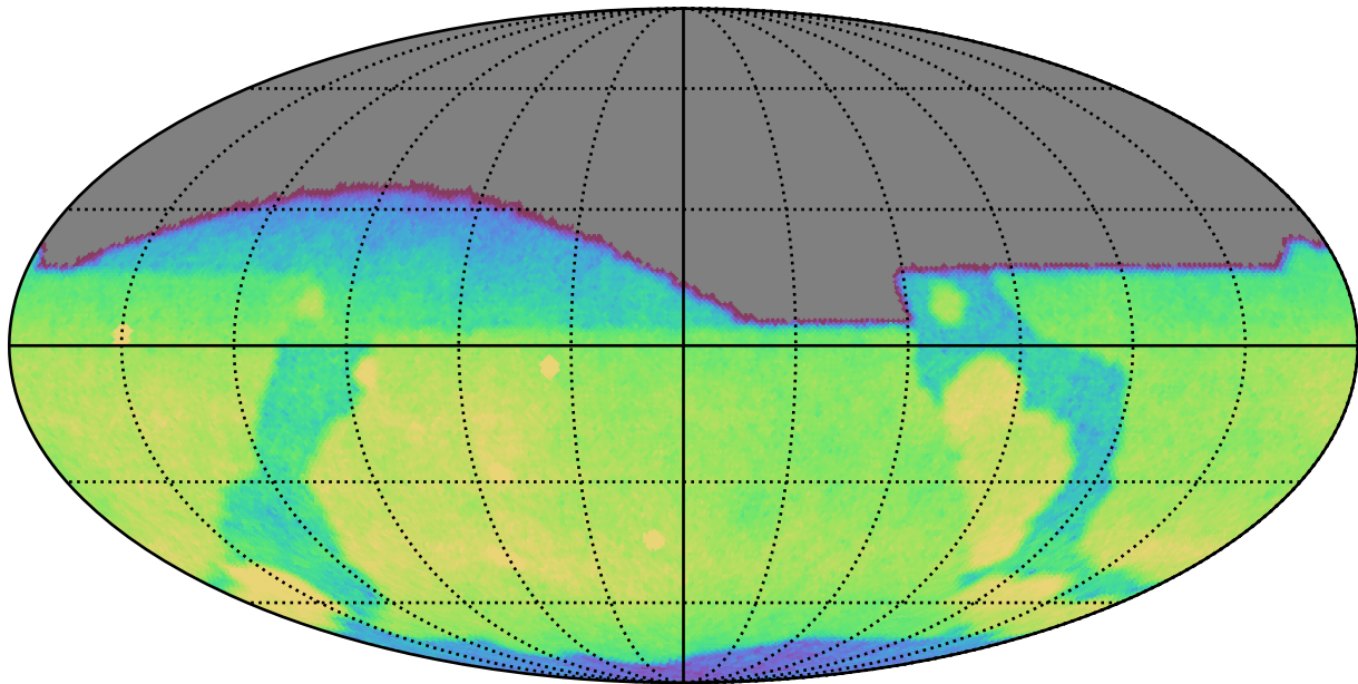
early_ss_template_fpextra3.0_v3.4_10yrs All sky g band: CoaddM5
